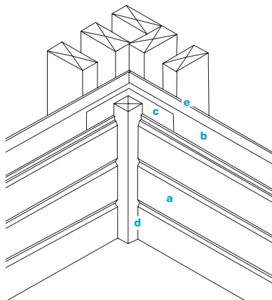
Inside Corner Detail-a
